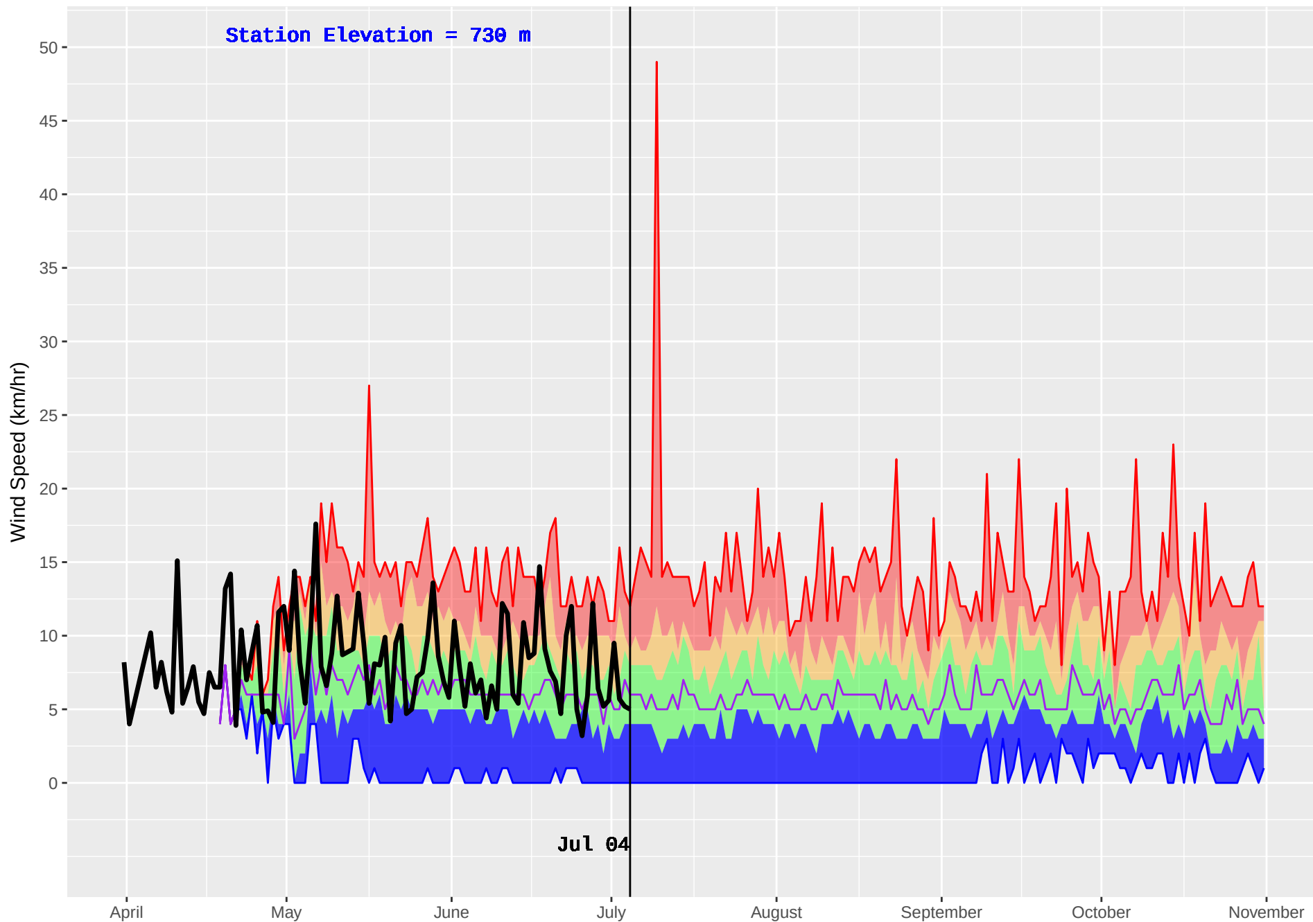
BOYA LAKE (445) : Historical (1985–2016) and Current (2018) Noon Wind Speed
