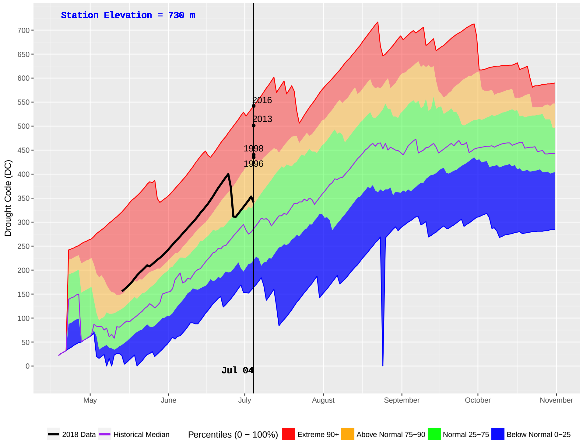
BOYA LAKE (445) : Historical (1985–2016) and Current (2018) Noon Drought Code (DC)
