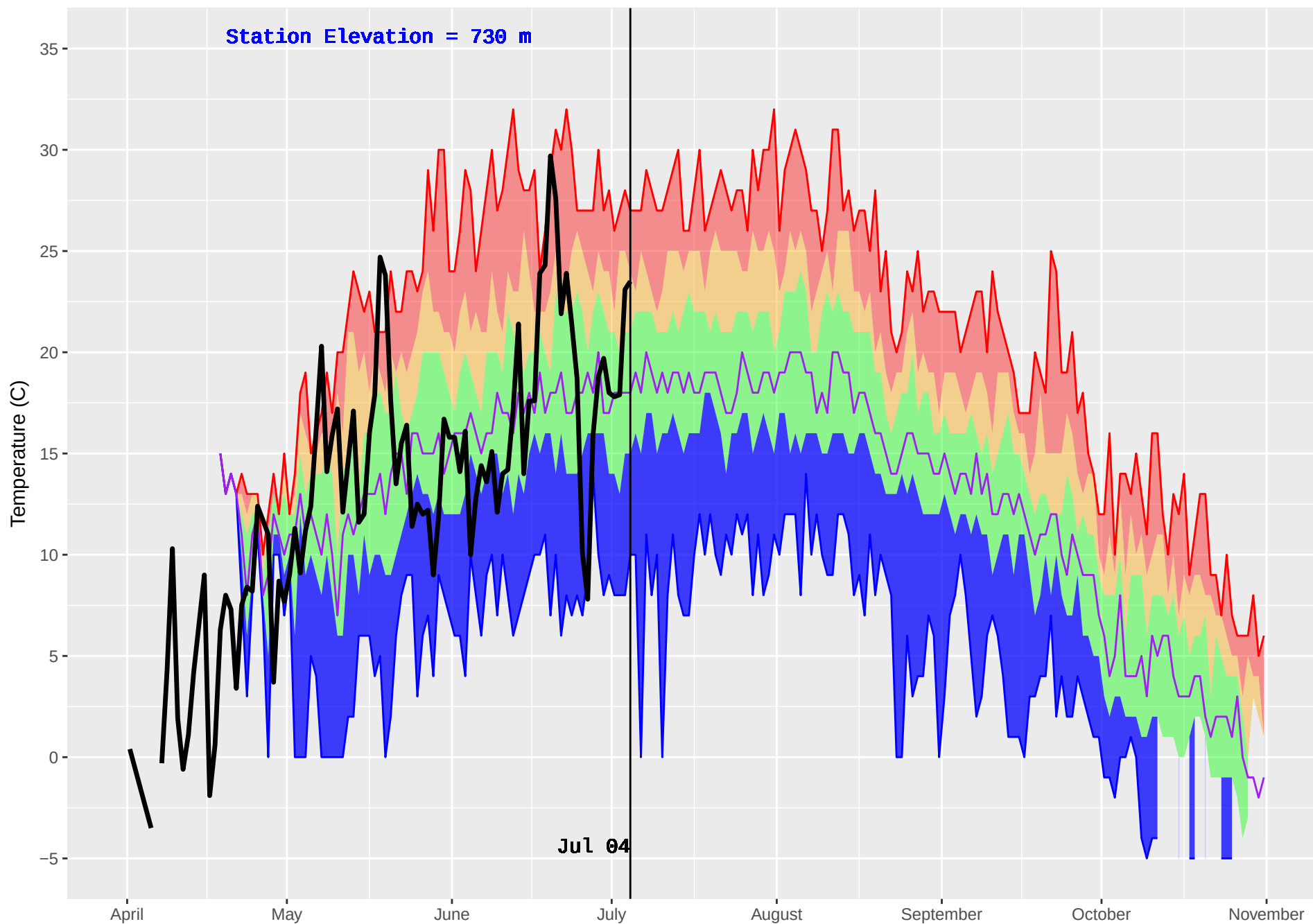
BOYA LAKE (445) : Historical (1985–2016) and Current (2018) Noon Temperature
