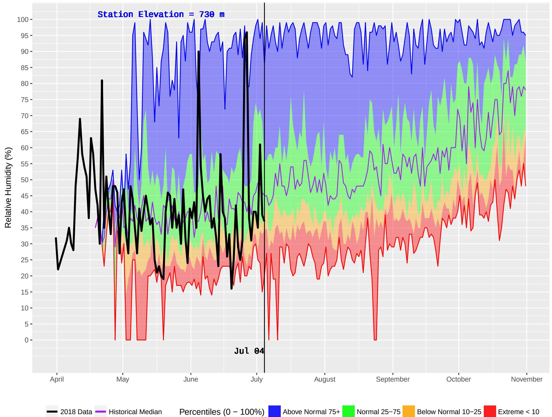
BOYA LAKE (445) : Historical (1985–2016) and Current (2018) Noon Relative Humidity
